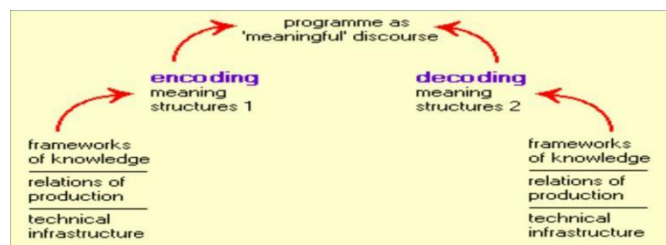
Gambar 1. Model Encoding-Decoding
